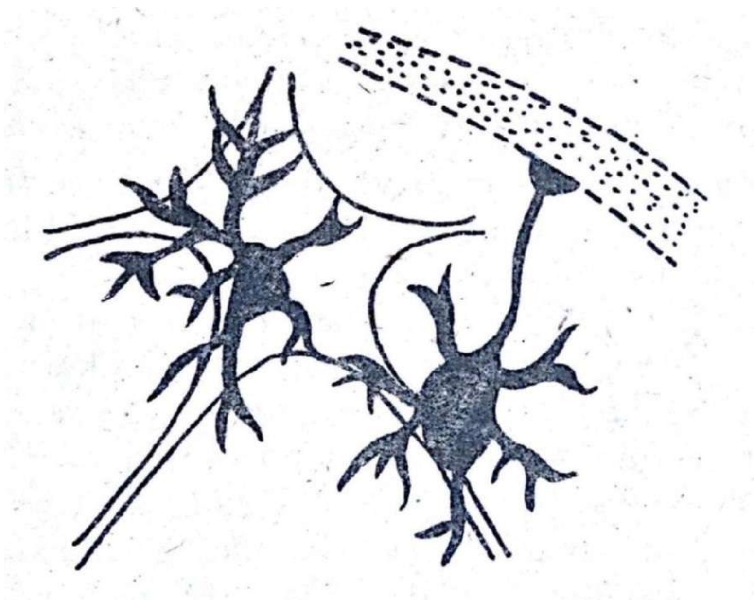
Nơ-ron
