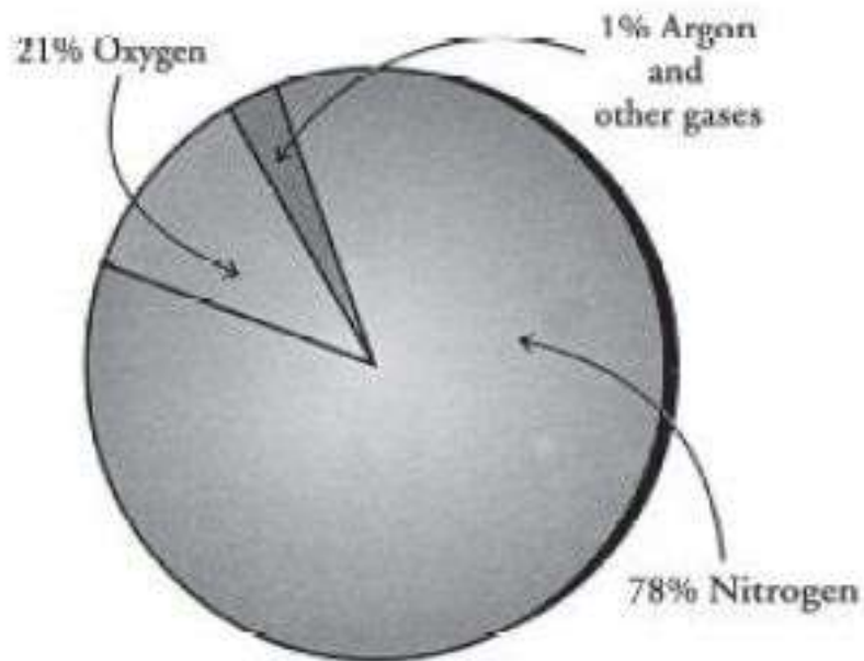
Earth's atmosphere
