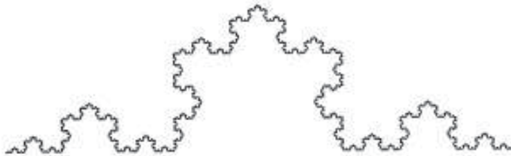
Benoit Mandelbrot
