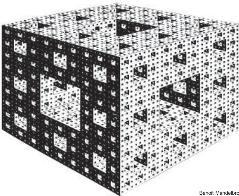
Benoit Mandelbrot
